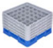
RWP1623BL Rack | 36 Compartments 19.7"L x 19.7"W x 12.1"H 1 CT
